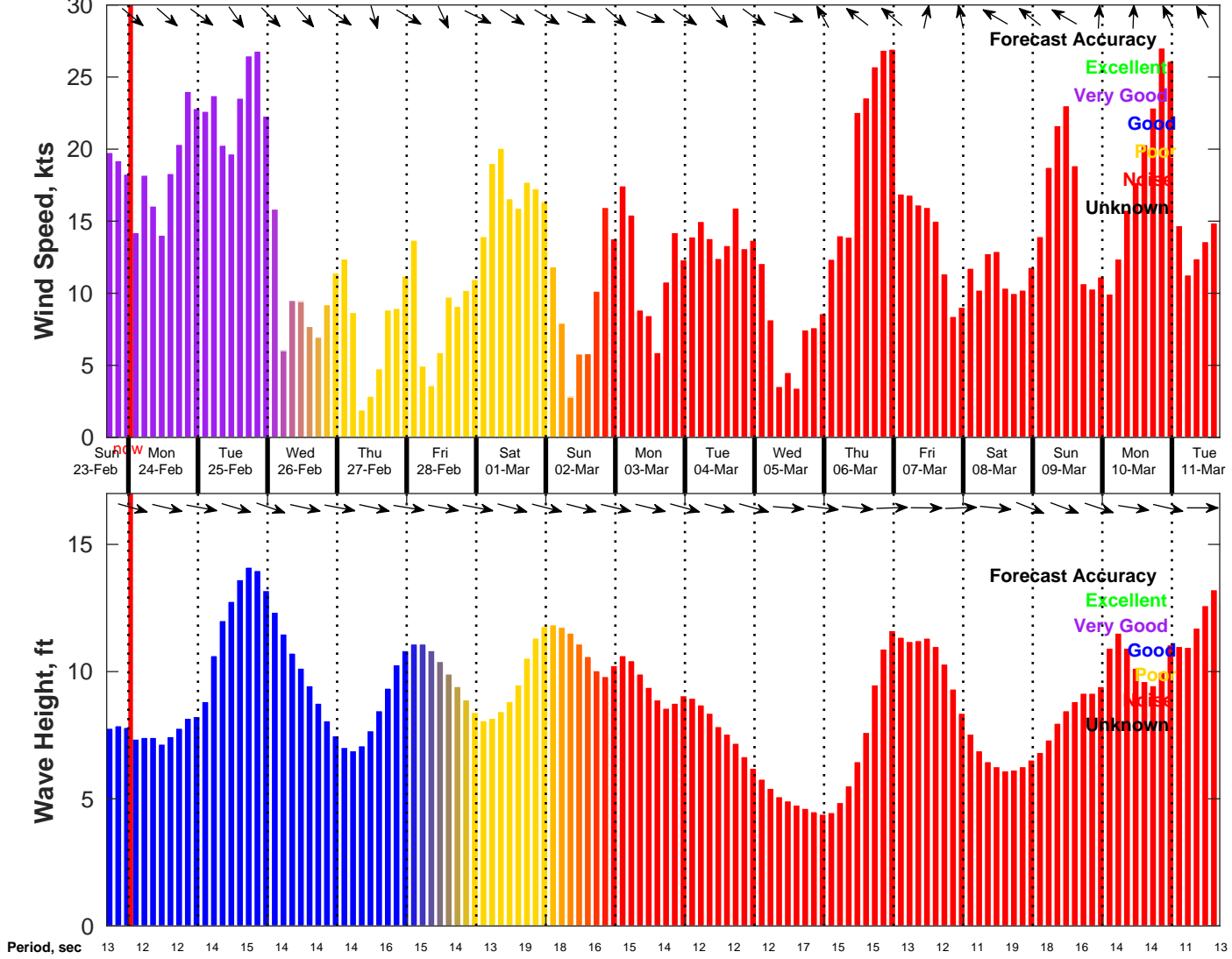
Wind & Wave Forecast for NDBC 46028 from 23-Feb-2025 16:00:00 to 11-Mar-2025 16:00:00
