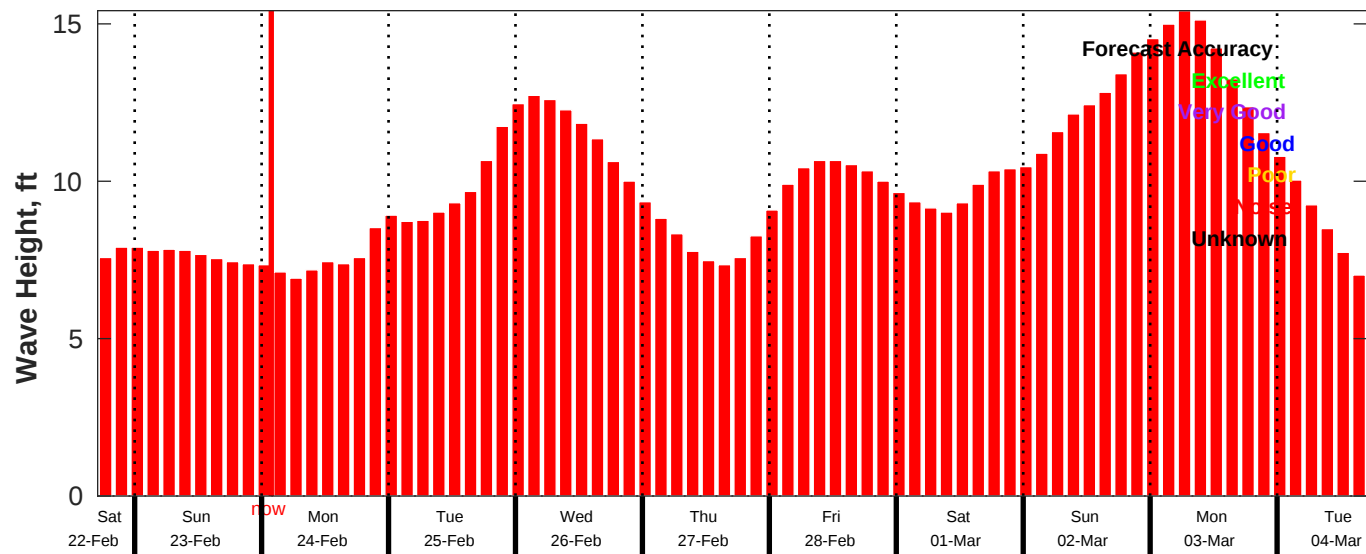
CMEMS Wave Forecast for NDBC 46053 from 22-Feb-2025 17:00:00 to 04-Mar-2025 17:00:00
