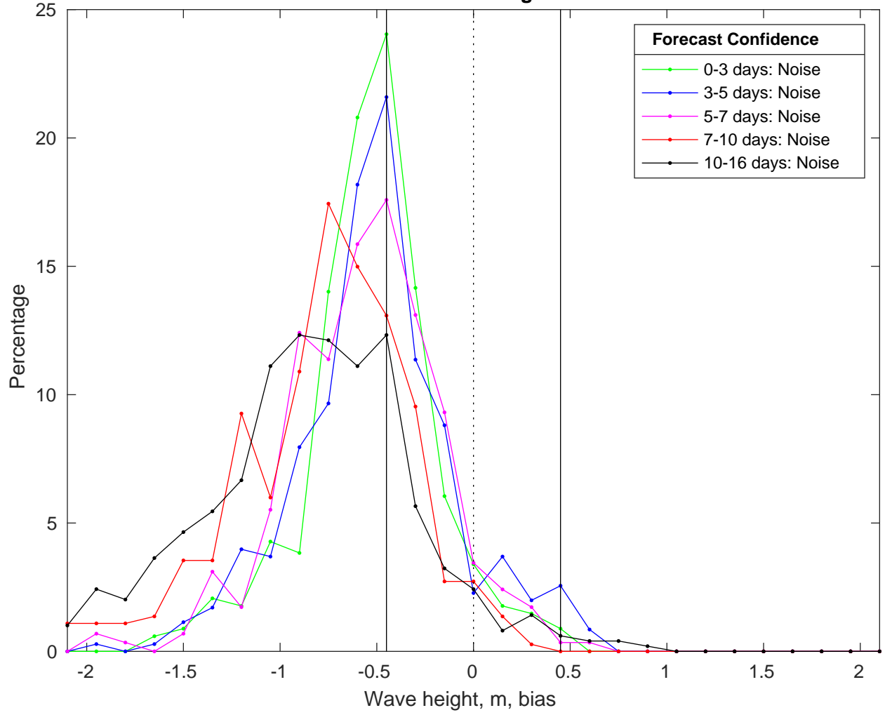
NDBC 46054 vs GFS Waves Bias Histogram: 24-Feb-2025
