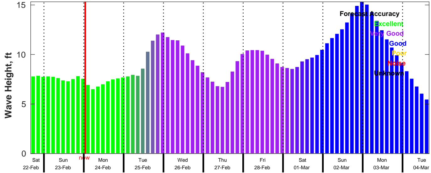
CMEMS Wave Forecast for NDBC 46054 from 22-Feb-2025 16:00:00 to 04-Mar-2025 16:00:00
