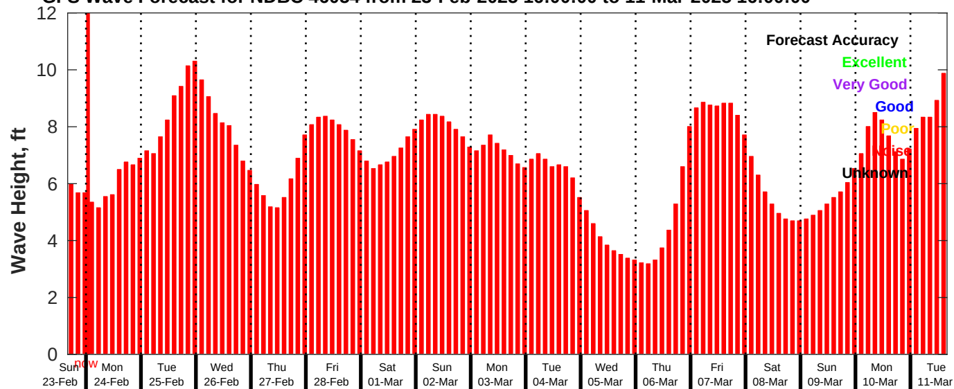
GFS Wave Forecast for NDBC 46054 from 23-Feb-2025 16:00:00 to 11-Mar-2025 16:00:00
