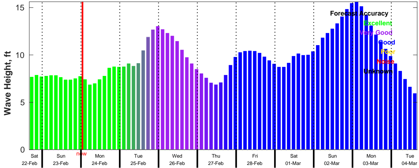
CMEMS Wave Forecast for NDBC 46069 from 22-Feb-2025 16:00:00 to 04-Mar-2025 16:00:00
