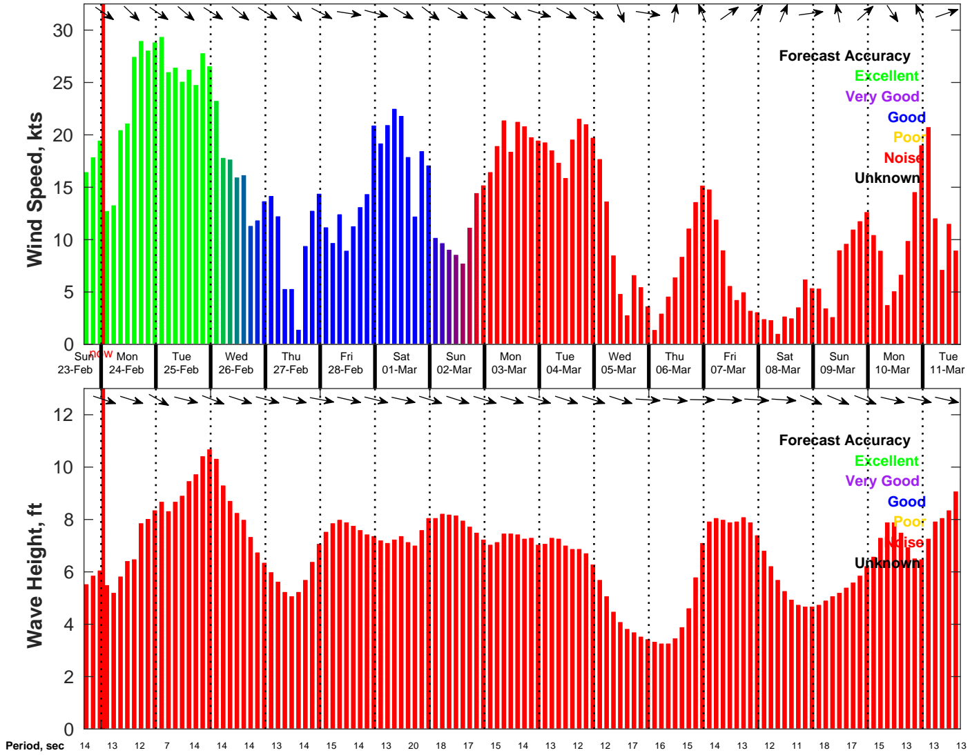
Wind & Wave Forecast for NDBC 46069 from 23-Feb-2025 16:00:00 to 11-Mar-2025 16:00:00
