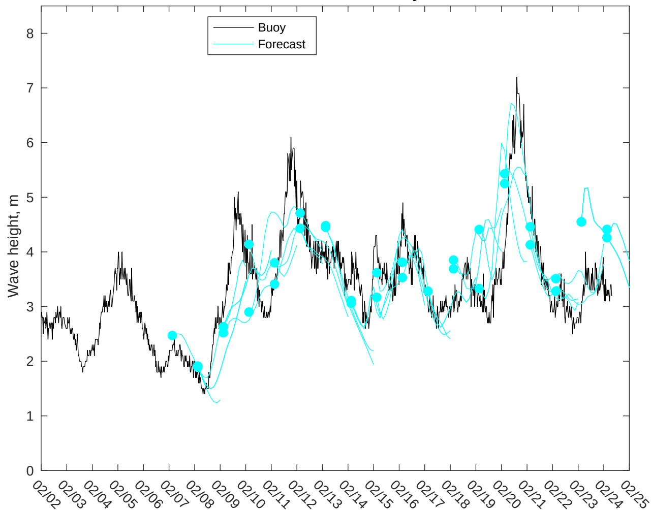
NDBC 46246 vs CMEMS Waves: 5 to 7 day forecast
