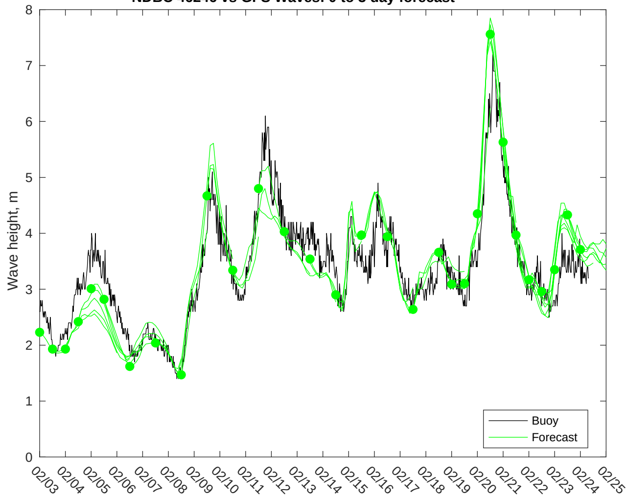
NDBC 46246 vs GFS Waves: 0 to 3 day forecast
