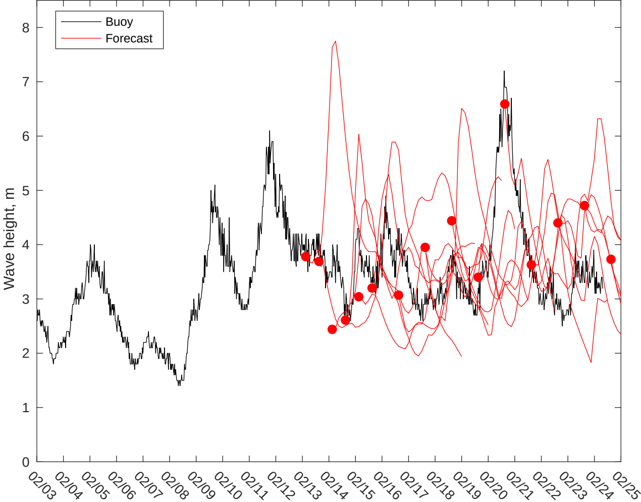
NDBC 46246 vs GFS Waves: 10 to 16 day forecast
