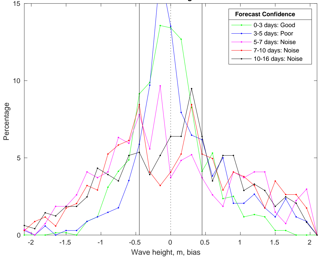
NDBC 46246 vs GFS Waves Bias Histogram: 24-Feb-2025
