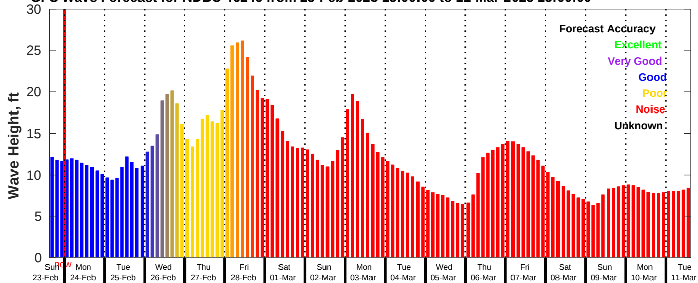
GFS Wave Forecast for NDBC 46246 from 23-Feb-2025 15:00:00 to 11-Mar-2025 15:00:00
