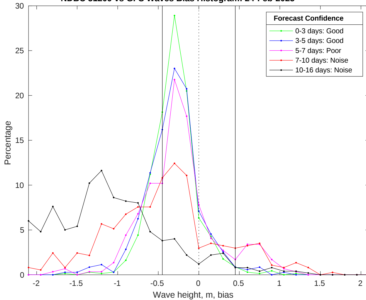
NDBC 51209 vs GFS Waves Bias Histogram: 24-Feb-2025
