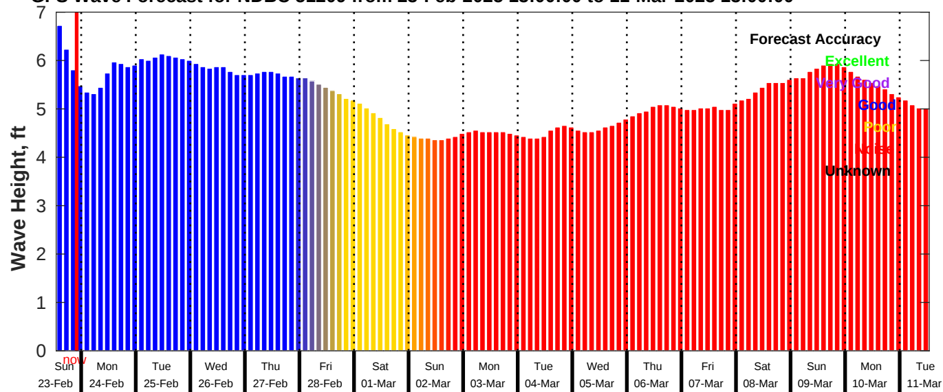
GFS Wave Forecast for NDBC 51209 from 23-Feb-2025 13:00:00 to 11-Mar-2025 13:00:00
