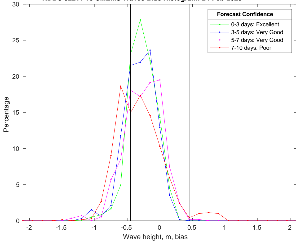
NDBC 52211 vs CMEMS Waves Bias Histogram: 24-Feb-2025
