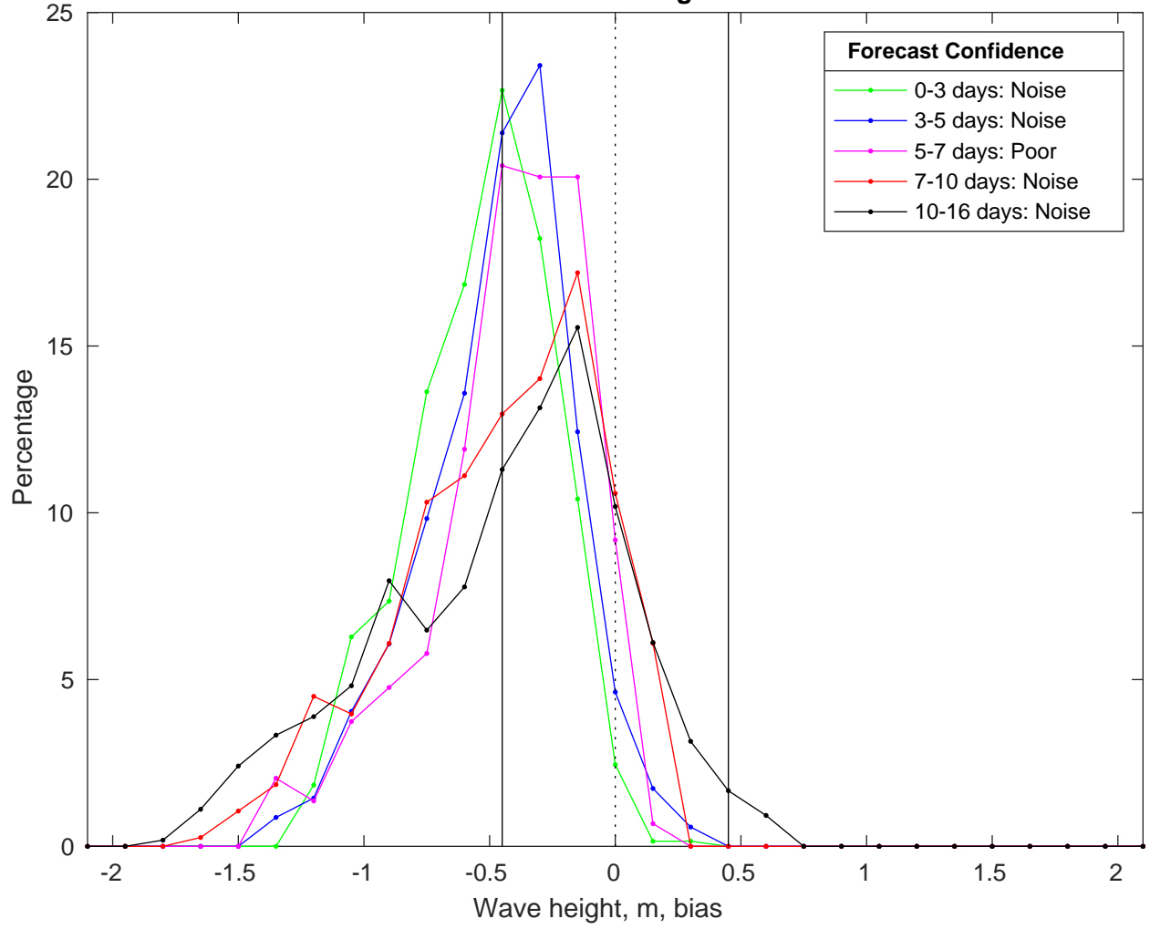
NDBC 52213 vs GFS Waves Bias Histogram: 24-Feb-2025
