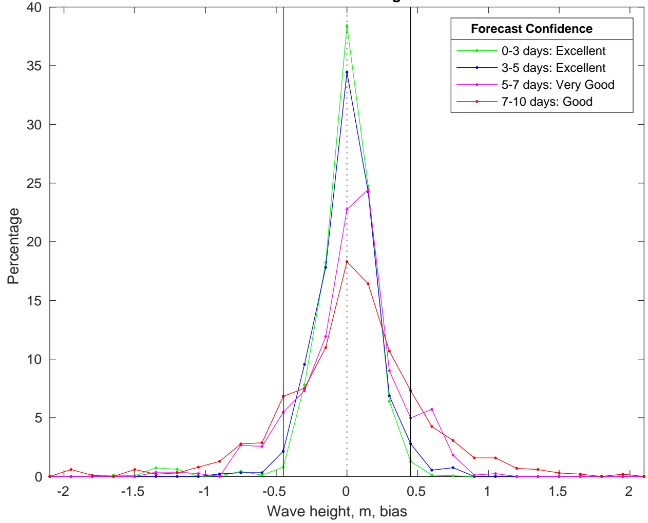
NDBC 41004 vs CMEMS Waves Bias Histogram: 25-Feb-2025
