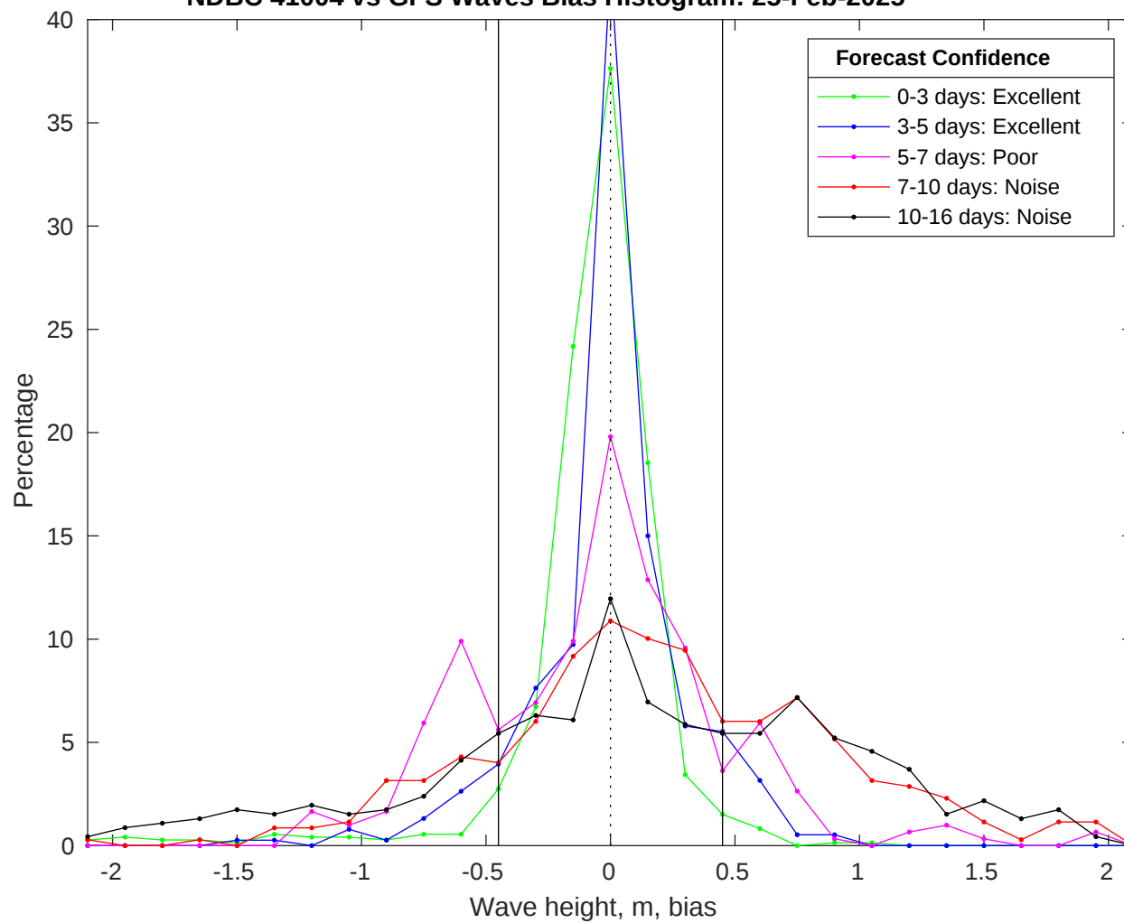
NDBC 41004 vs GFS Waves Bias Histogram: 25-Feb-2025
