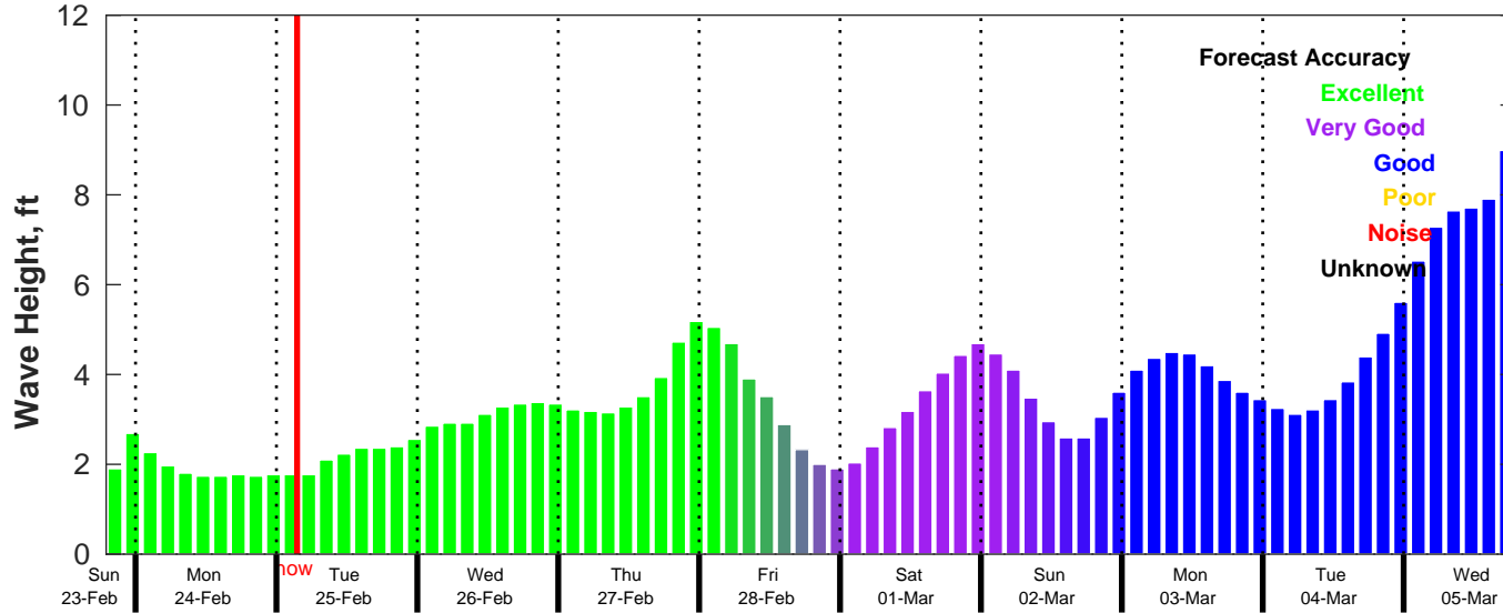
CMEMS Wave Forecast for NDBC 41004 from 23-Feb-2025 19:00:00 to 05-Mar-2025 19:00:00
