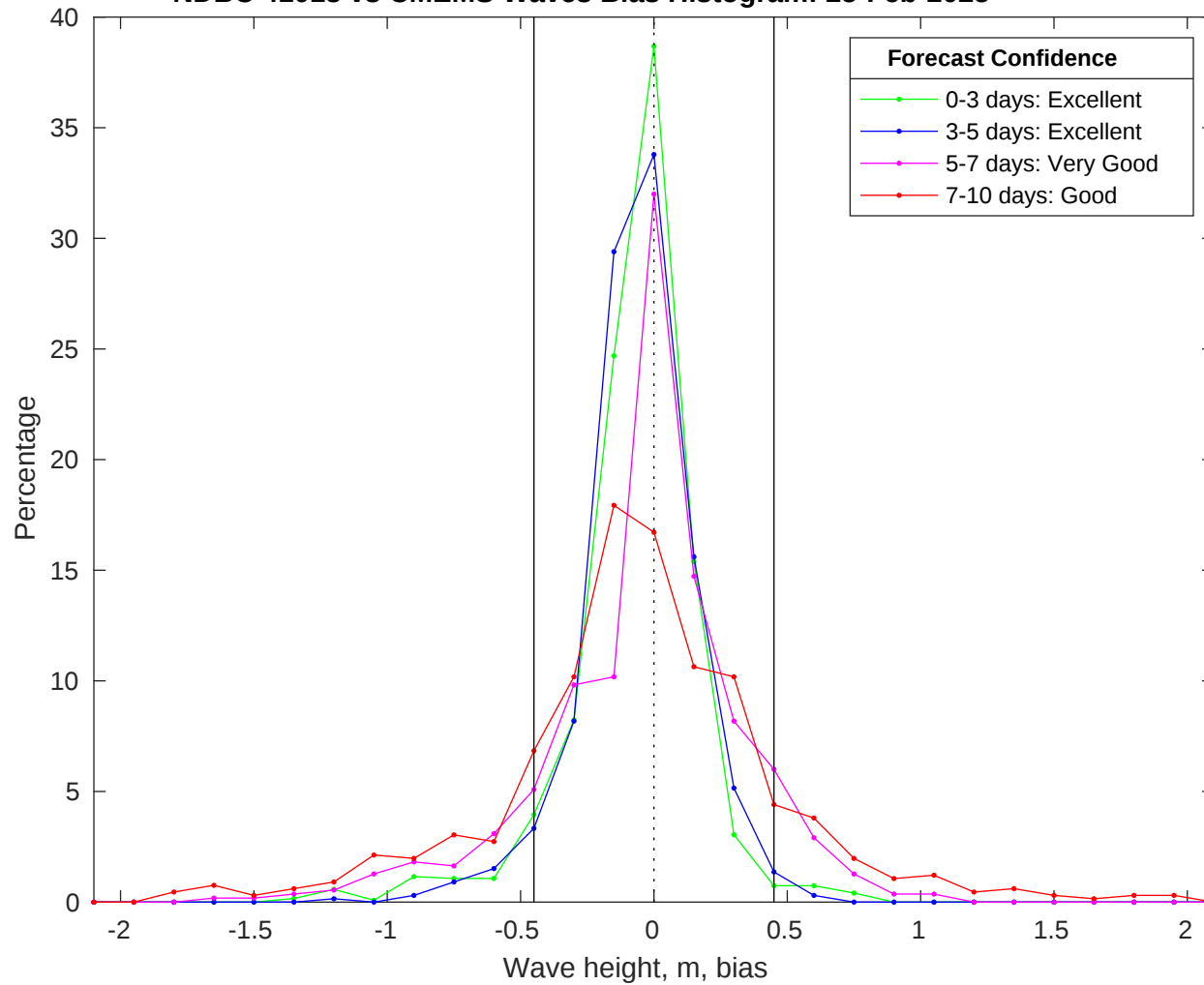
NDBC 41013 vs CMEMS Waves Bias Histogram: 25-Feb-2025
