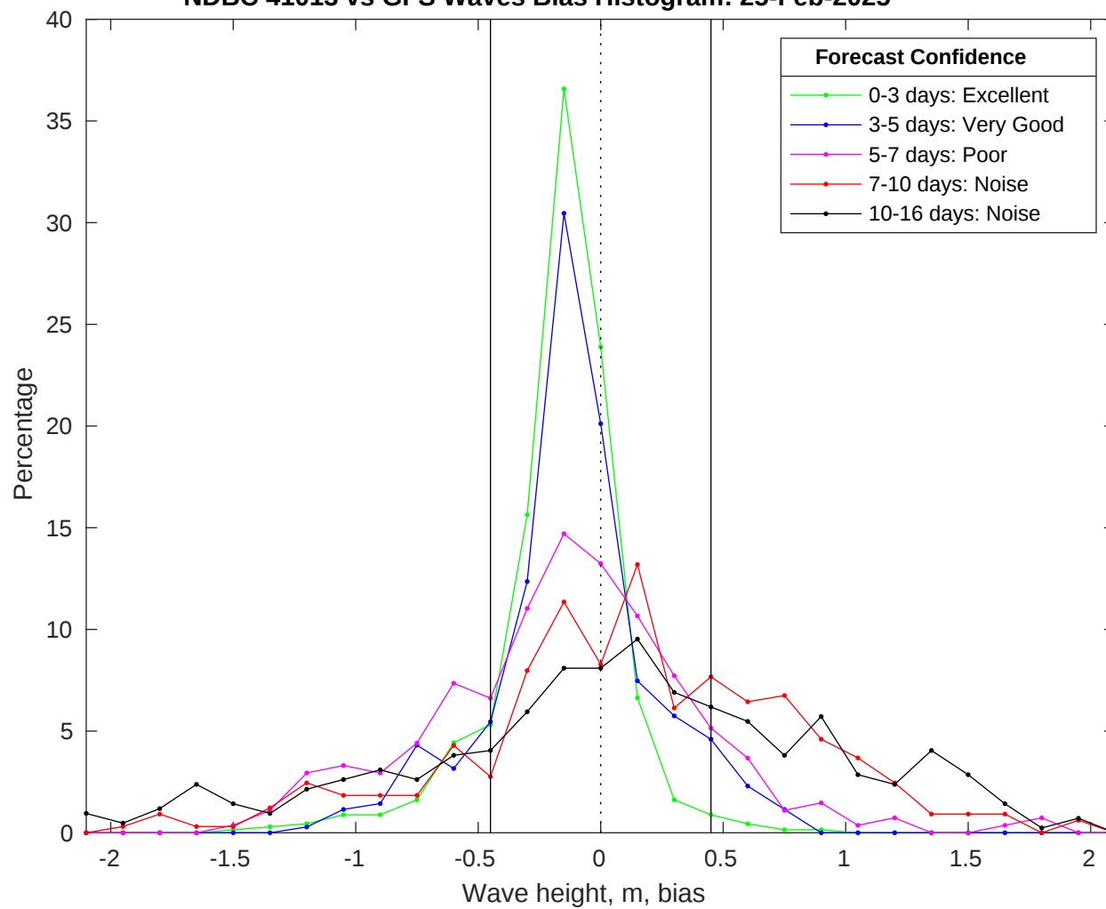
NDBC 41013 vs GFS Waves Bias Histogram: 25-Feb-2025
