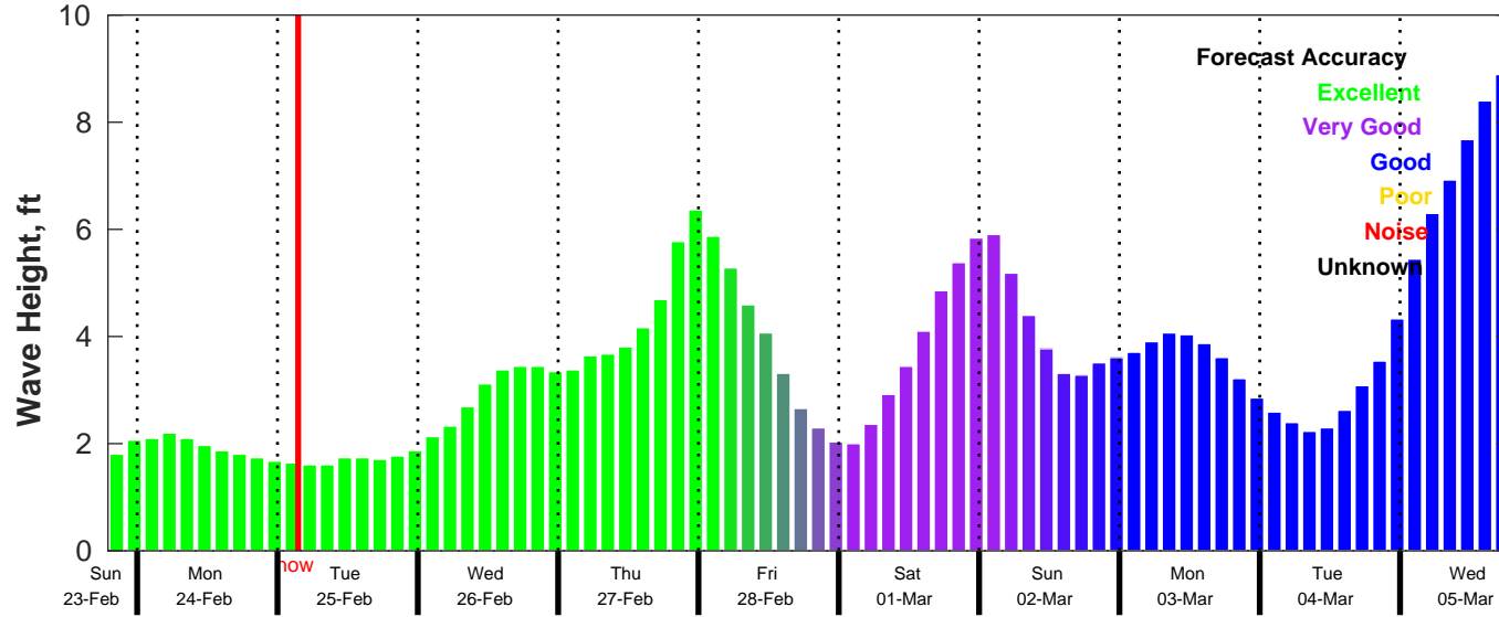
CMEMS Wave Forecast for NDBC 41013 from 23-Feb-2025 19:00:00 to 05-Mar-2025 19:00:00
