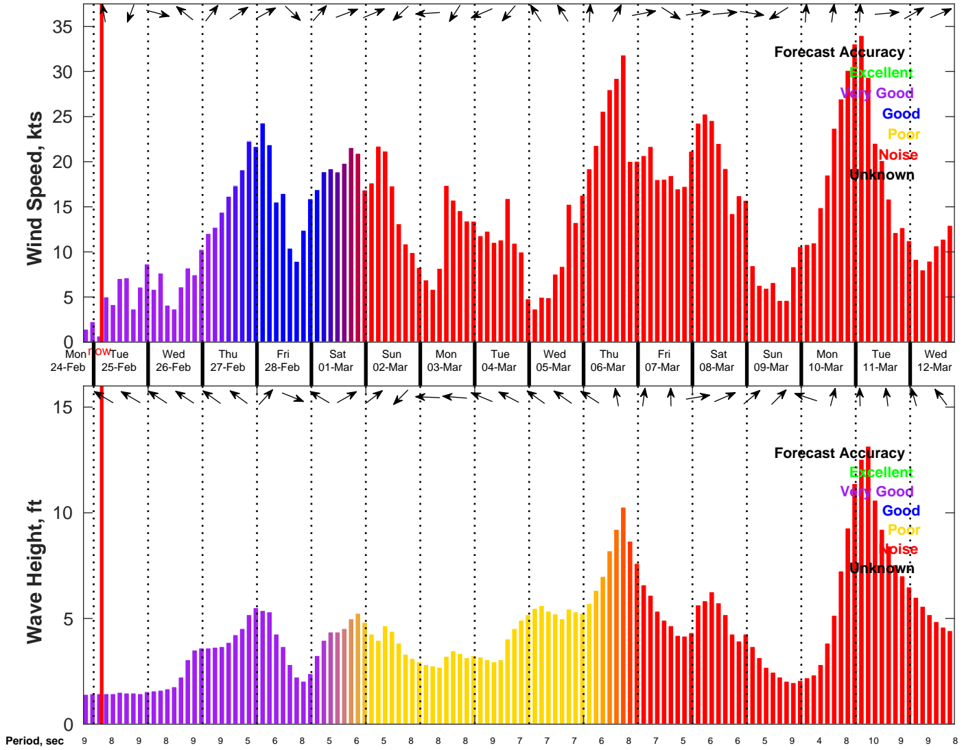
Wind & Wave Forecast for NDBC 41013 from 24-Feb-2025 19:00:00 to 12-Mar-2025 19:00:00
