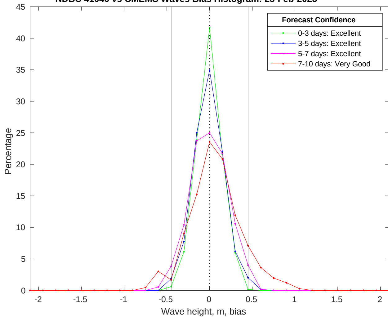
NDBC 41040 vs CMEMS Waves Bias Histogram: 25-Feb-2025
