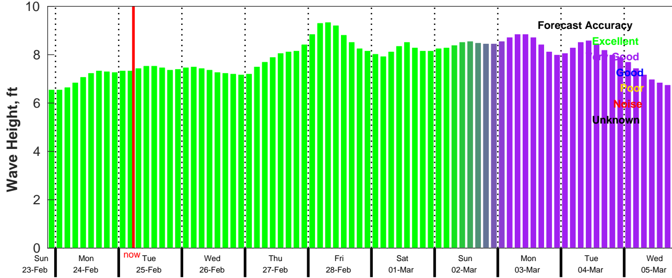
CMEMS Wave Forecast for NDBC 41040 from 23-Feb-2025 21:00:00 to 05-Mar-2025 21:00:00
