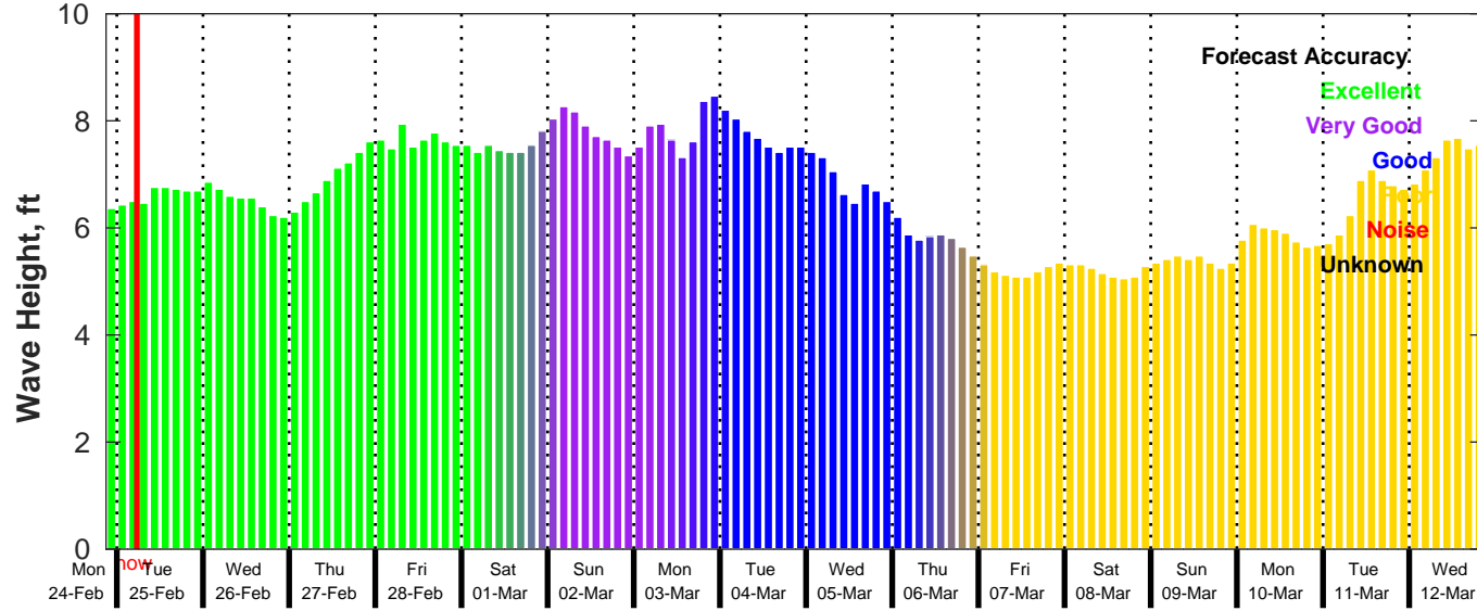
GFS Wave Forecast for NDBC 41040 from 24-Feb-2025 21:00:00 to 12-Mar-2025 21:00:00
