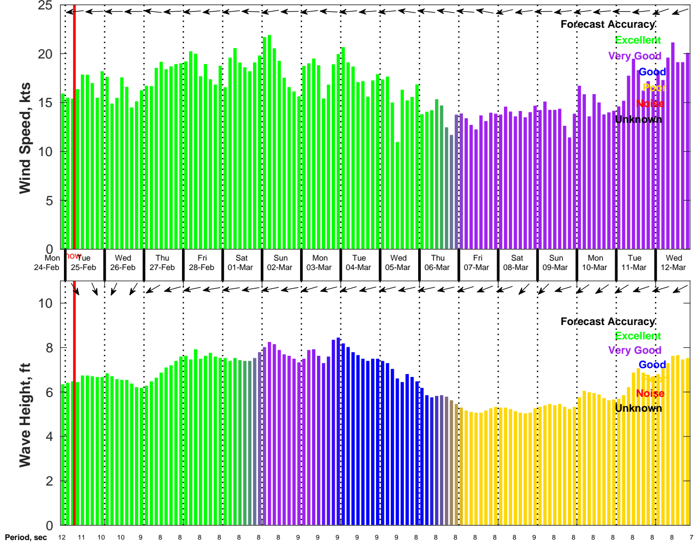
Wind & Wave Forecast for NDBC 41040 from 24-Feb-2025 21:00:00 to 12-Mar-2025 21:00:00
