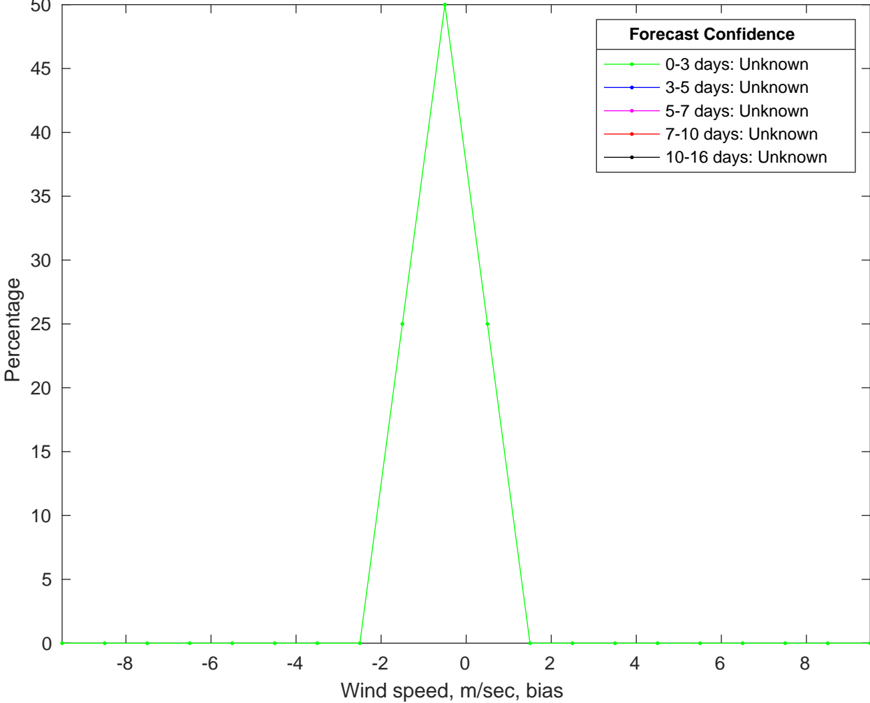
NDBC 42002 vs GFSWinds Bias Histogram: 07-Oct-2024
