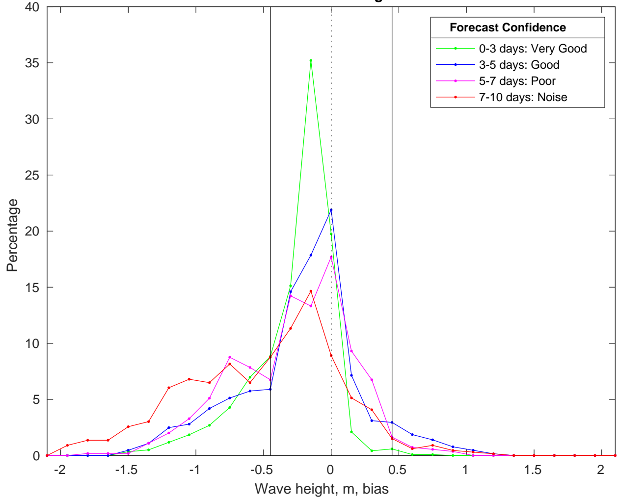
NDBC 42019 vs CMEMS Waves Bias Histogram: 25-Feb-2025
