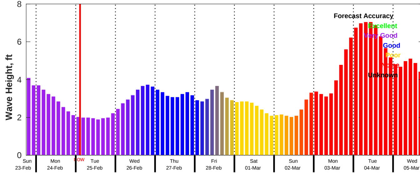
CMEMS Wave Forecast for NDBC 42019 from 23-Feb-2025 18:00:00 to 05-Mar-2025 18:00:00
