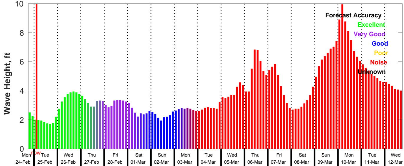
GFS Wave Forecast for NDBC 42019 from 24-Feb-2025 18:00:00 to 12-Mar-2025 18:00:00
