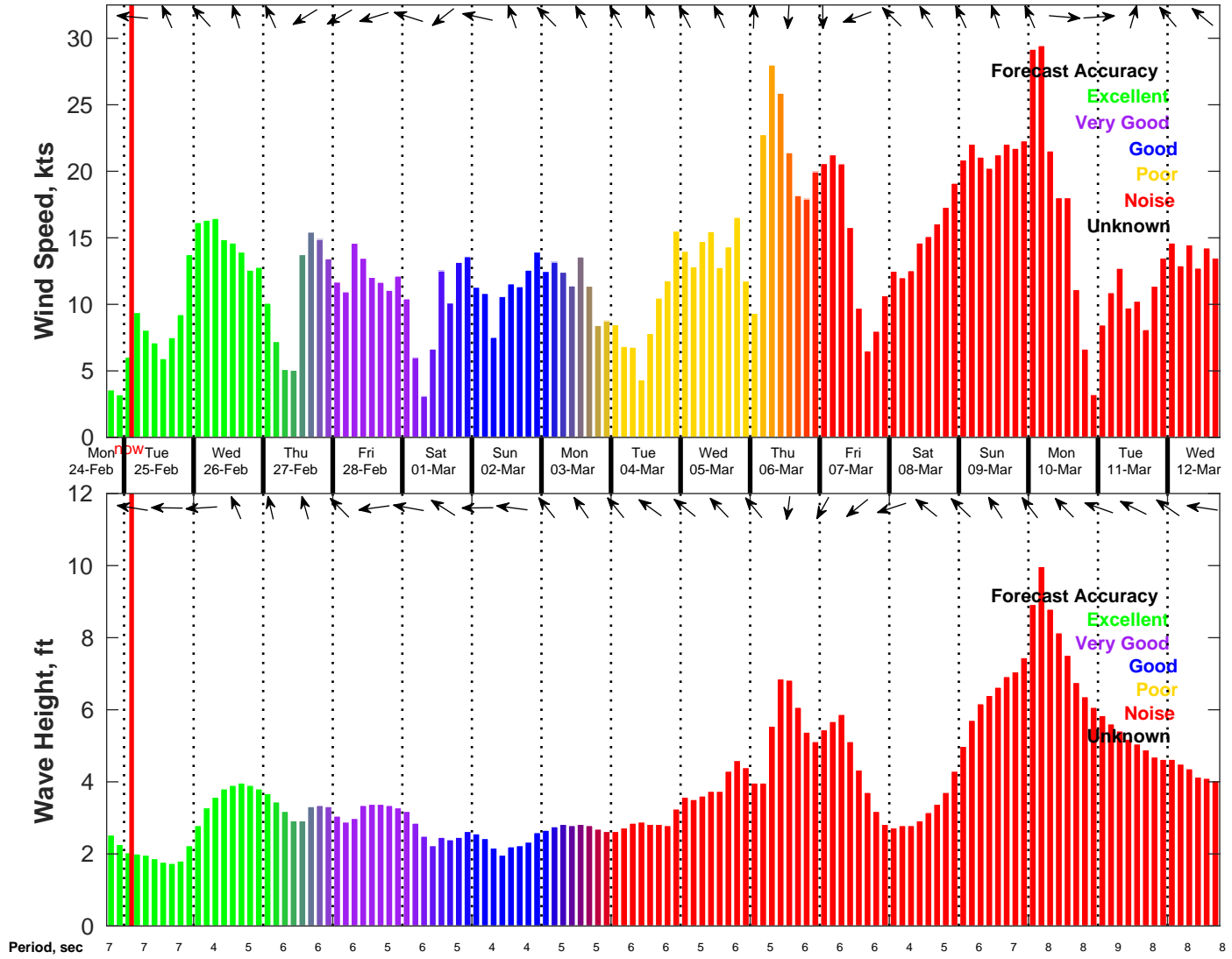
Wind & Wave Forecast for NDBC 42019 from 24-Feb-2025 18:00:00 to 12-Mar-2025 18:00:00
