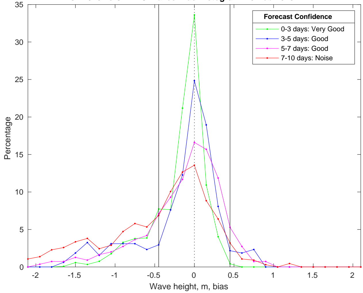
NDBC 42020 vs CMEMS Waves Bias Histogram: 25-Feb-2025
