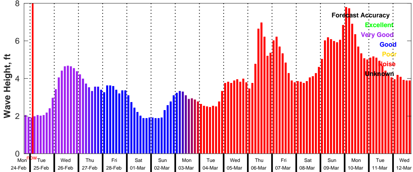
GFS Wave Forecast for NDBC 42020 from 24-Feb-2025 18:00:00 to 12-Mar-2025 18:00:00
