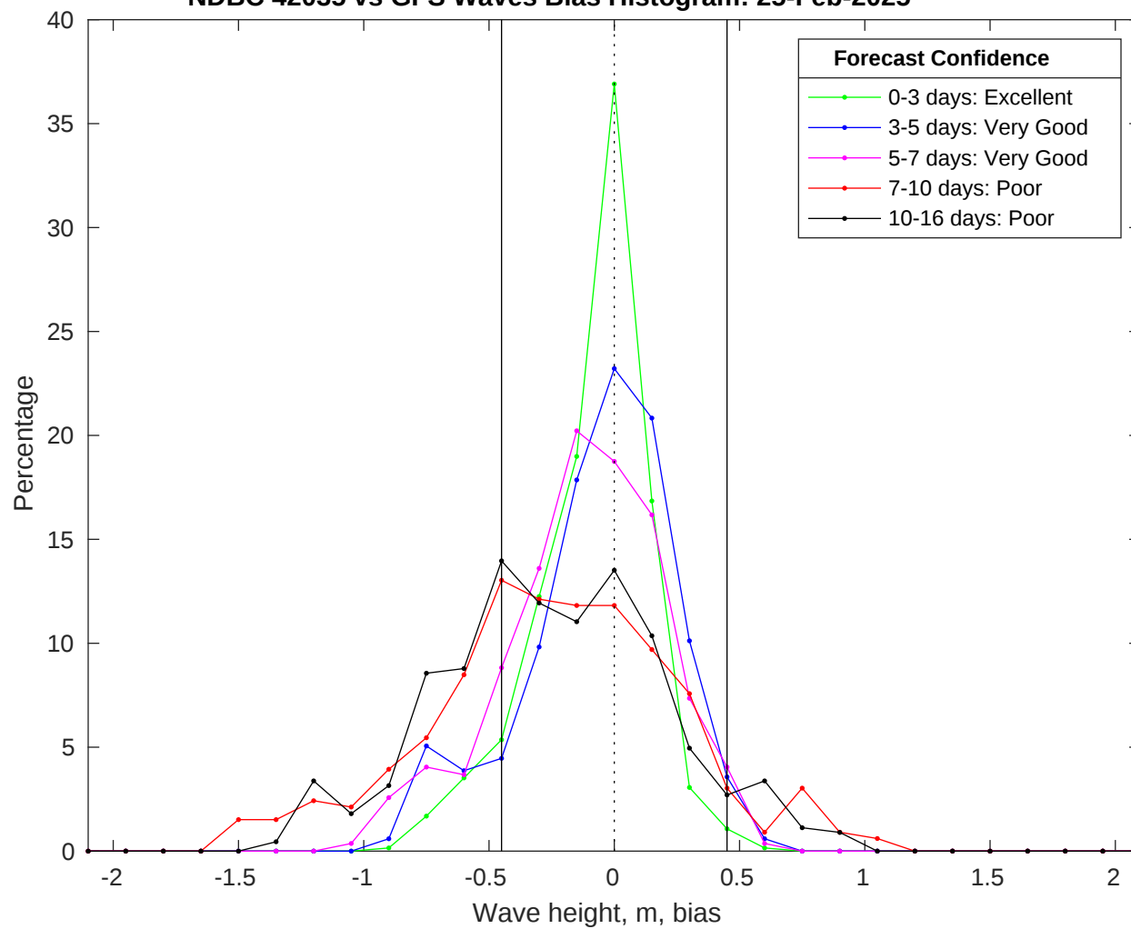
NDBC 42035 vs GFS Waves Bias Histogram: 25-Feb-2025
