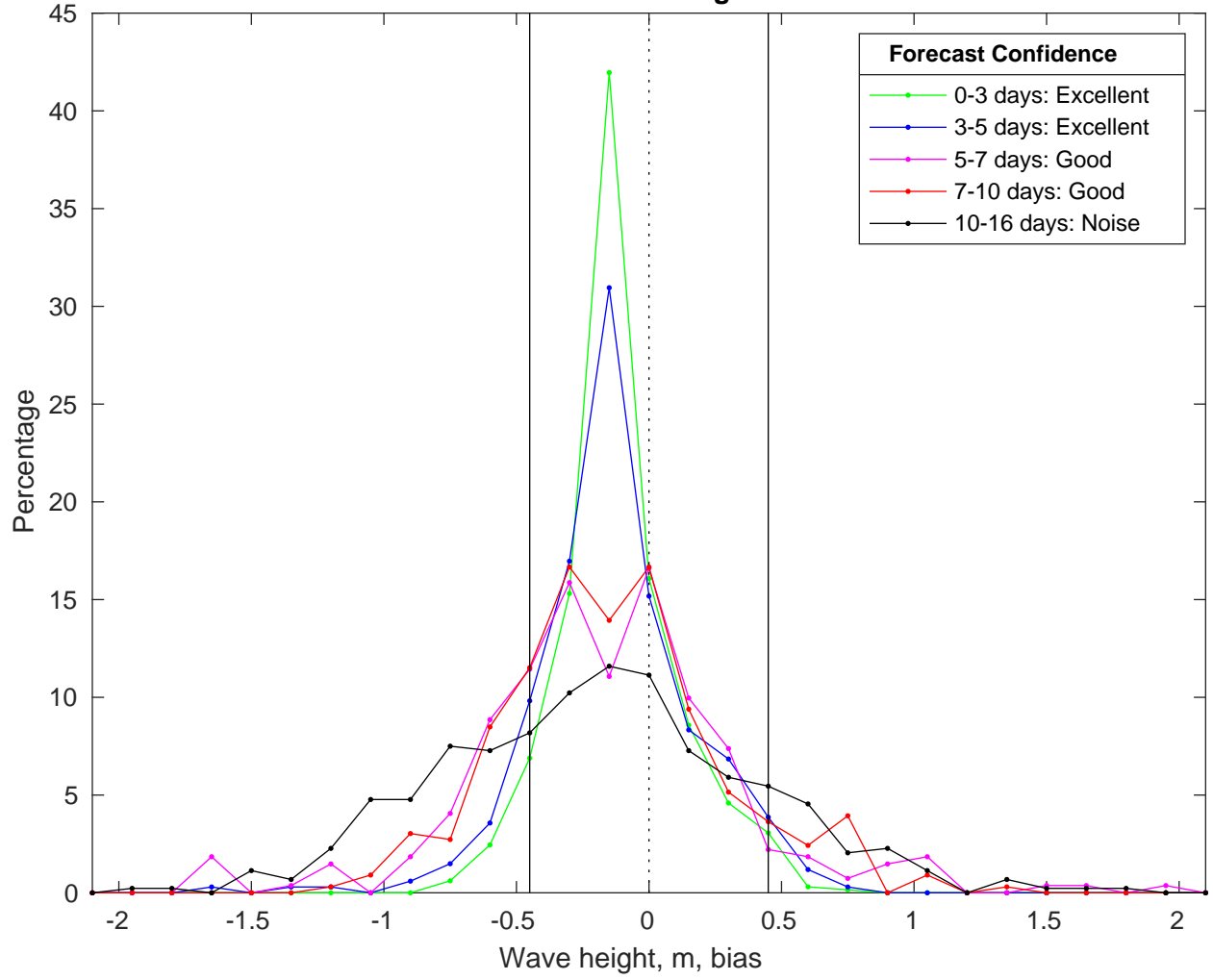
NDBC 42036 vs GFS Waves Bias Histogram: 25-Feb-2025
