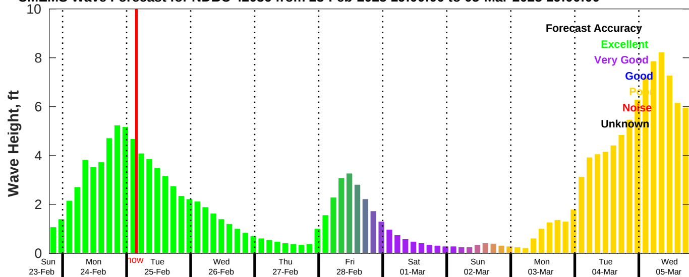
CMEMS Wave Forecast for NDBC 42036 from 23-Feb-2025 19:00:00 to 05-Mar-2025 19:00:00
