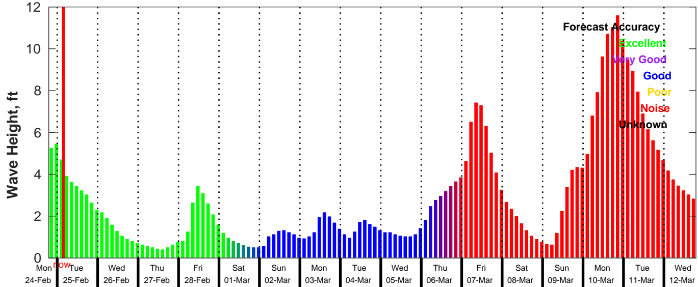
GFS Wave Forecast for NDBC 42036 from 24-Feb-2025 19:00:00 to 12-Mar-2025 19:00:00
