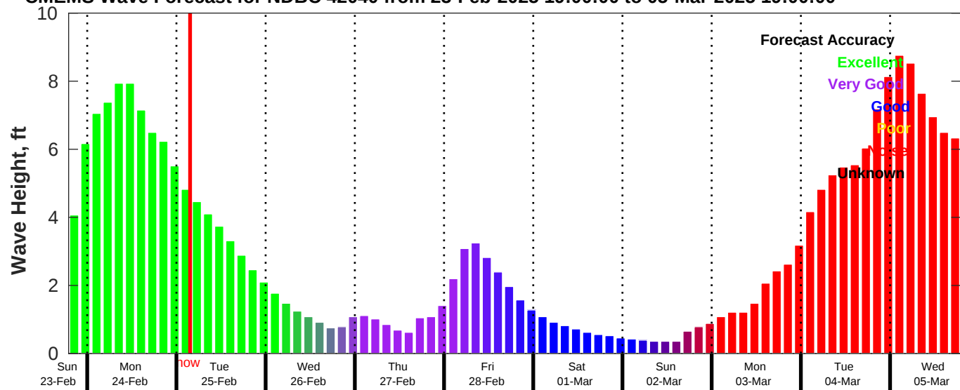
CMEMS Wave Forecast for NDBC 42040 from 23-Feb-2025 19:00:00 to 05-Mar-2025 19:00:00
