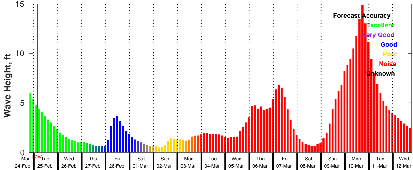
GFS Wave Forecast for NDBC 42040 from 24-Feb-2025 19:00:00 to 12-Mar-2025 19:00:00
