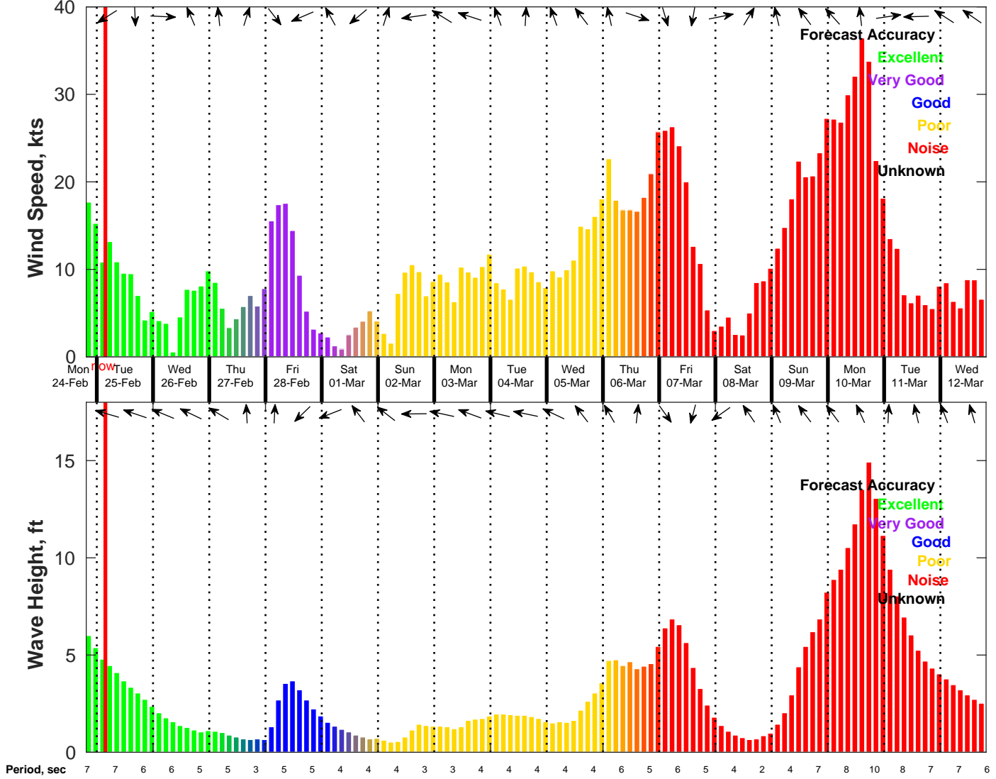
Wind & Wave Forecast for NDBC 42040 from 24-Feb-2025 19:00:00 to 12-Mar-2025 19:00:00
