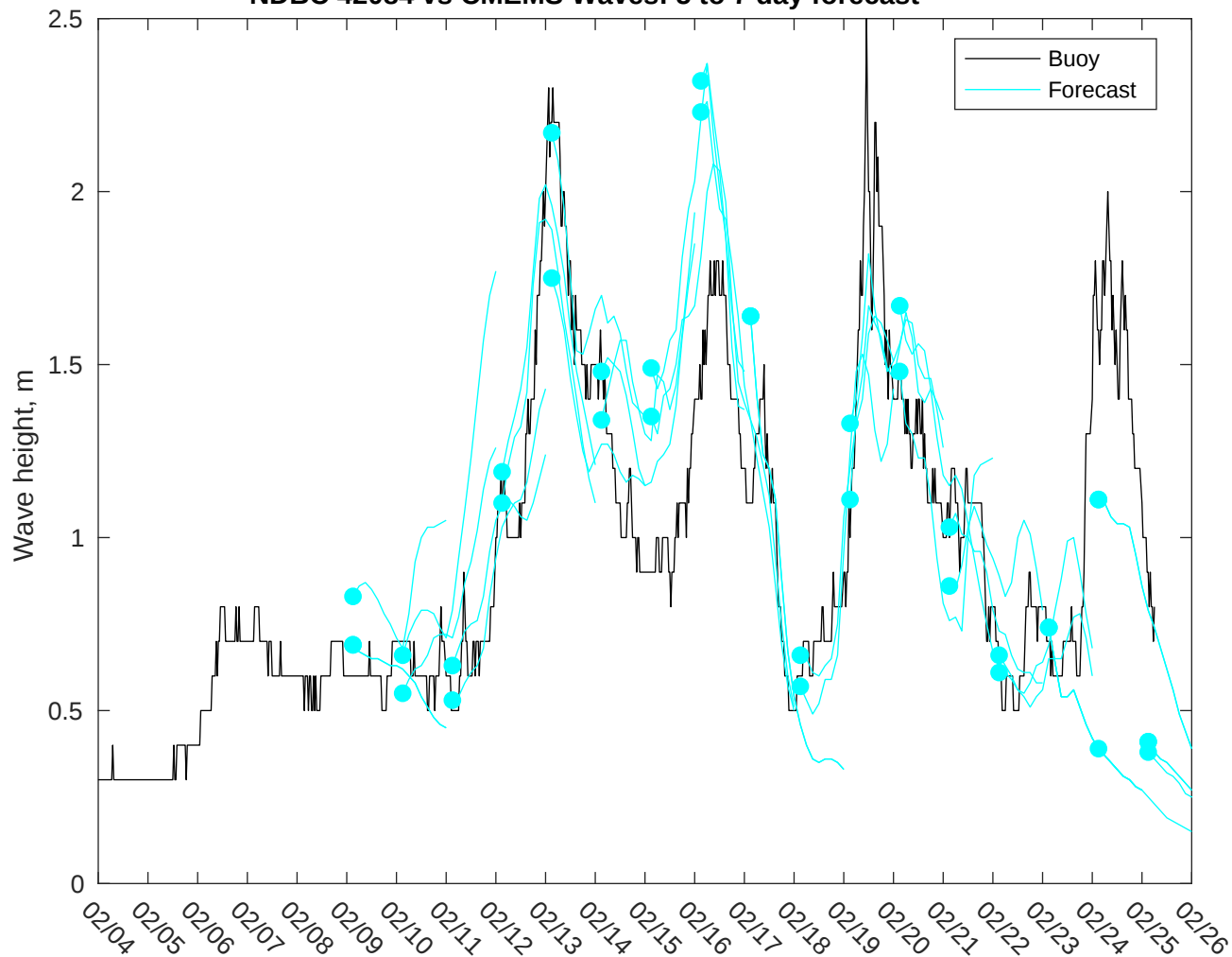
NDBC 42084 vs CMEMS Waves: 5 to 7 day forecast
