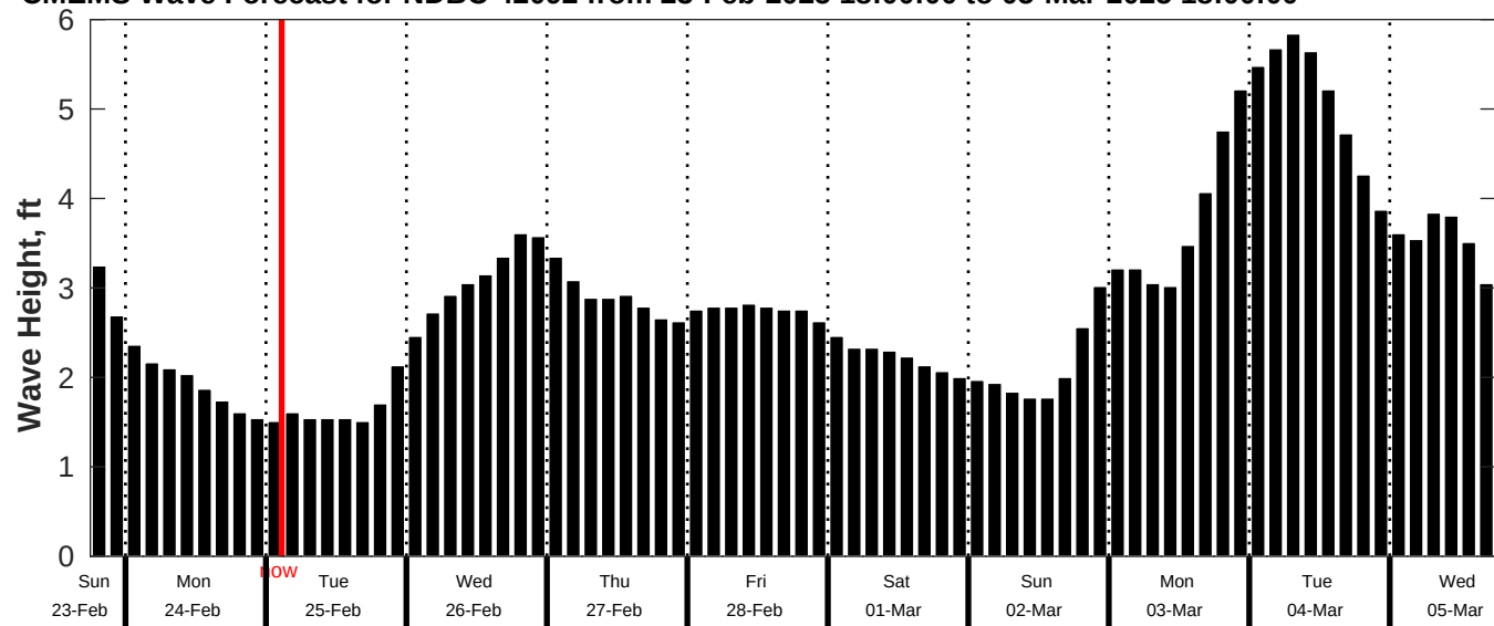
CMEMS Wave Forecast for NDBC 42092 from 23-Feb-2025 18:00:00 to 05-Mar-2025 18:00:00
