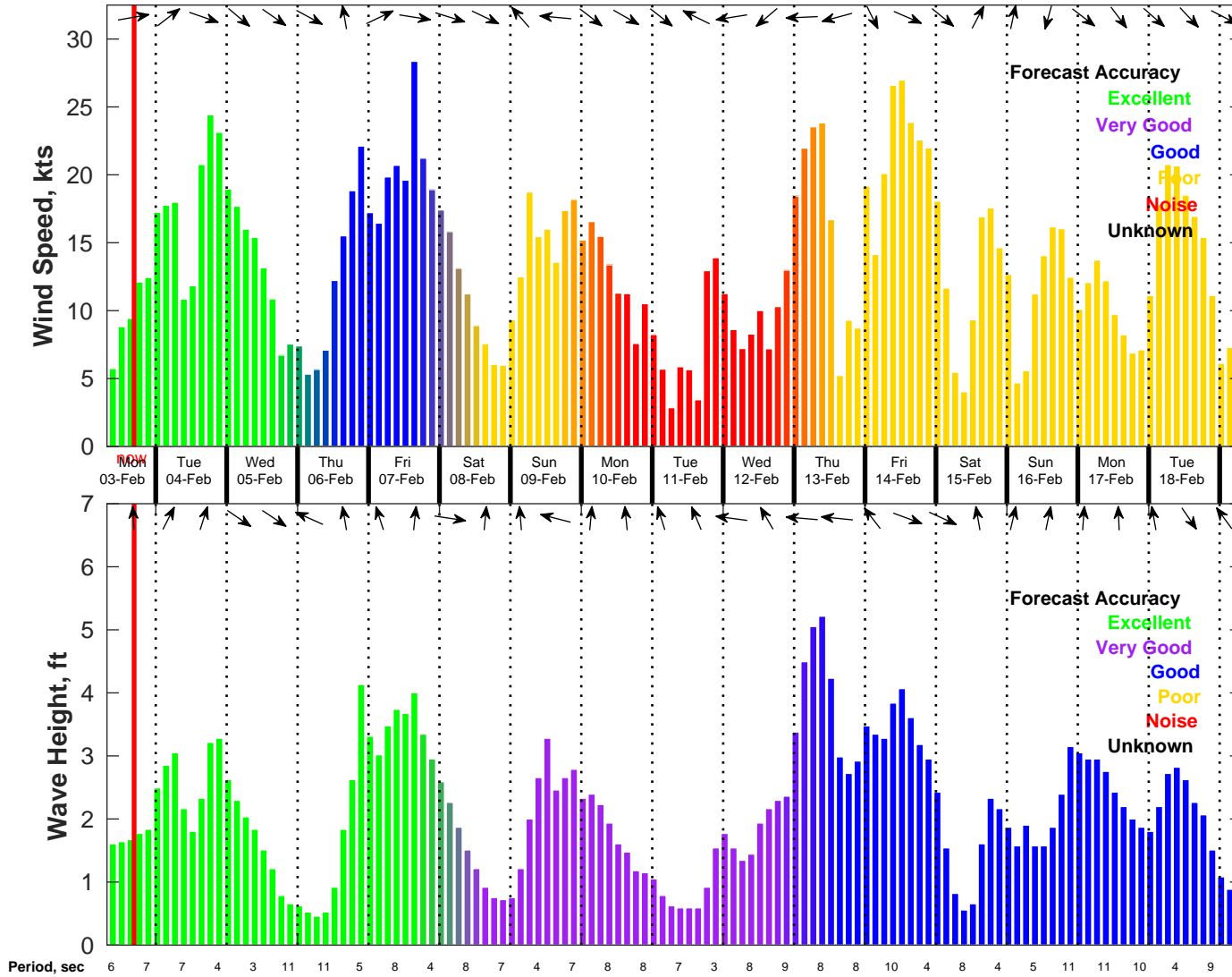
Wind & Wave Forecast for NDBC 44020 from 03-Feb-2025 08:00:00 to 19-Feb-2025 08:00:00
