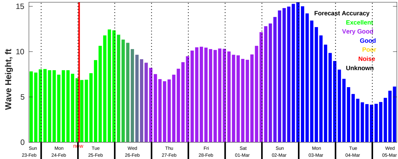
CMEMS Wave Forecast for NDBC 46011 from 23-Feb-2025 16:00:00 to 05-Mar-2025 16:00:00
