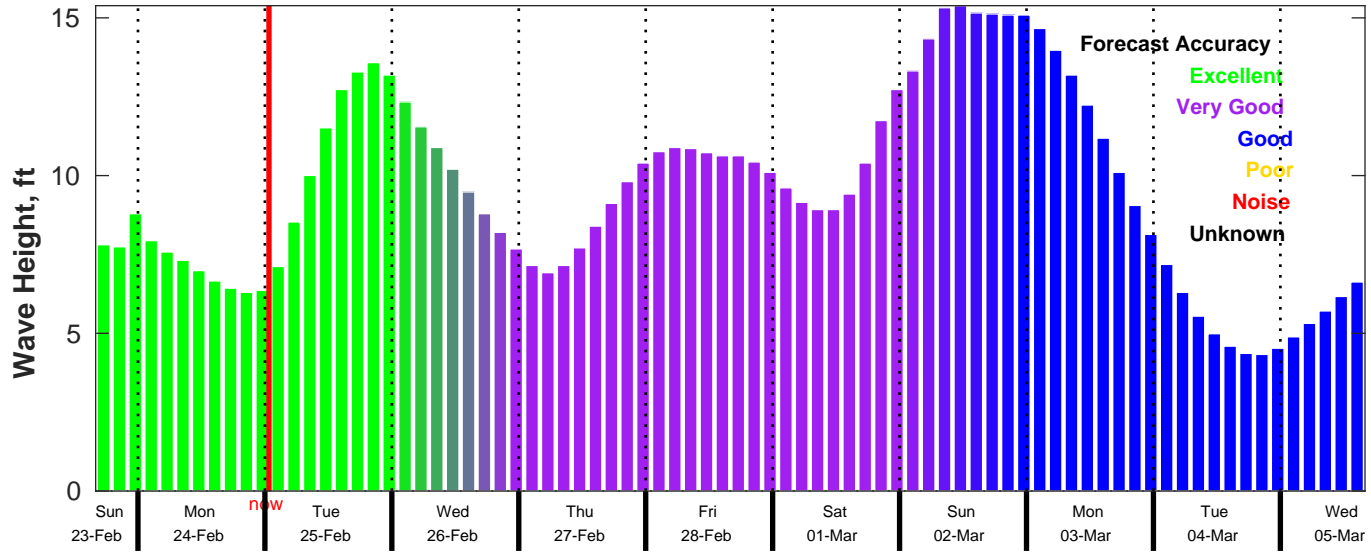
CMEMS Wave Forecast for NDBC 46028 from 23-Feb-2025 16:00:00 to 05-Mar-2025 16:00:00
