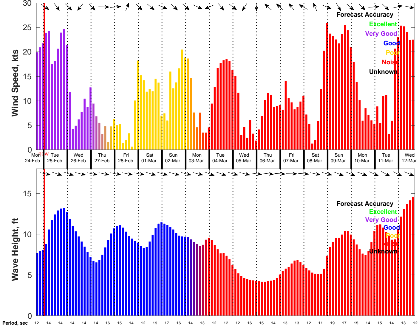
Wind & Wave Forecast for NDBC 46028 from 24-Feb-2025 16:00:00 to 12-Mar-2025 16:00:00
