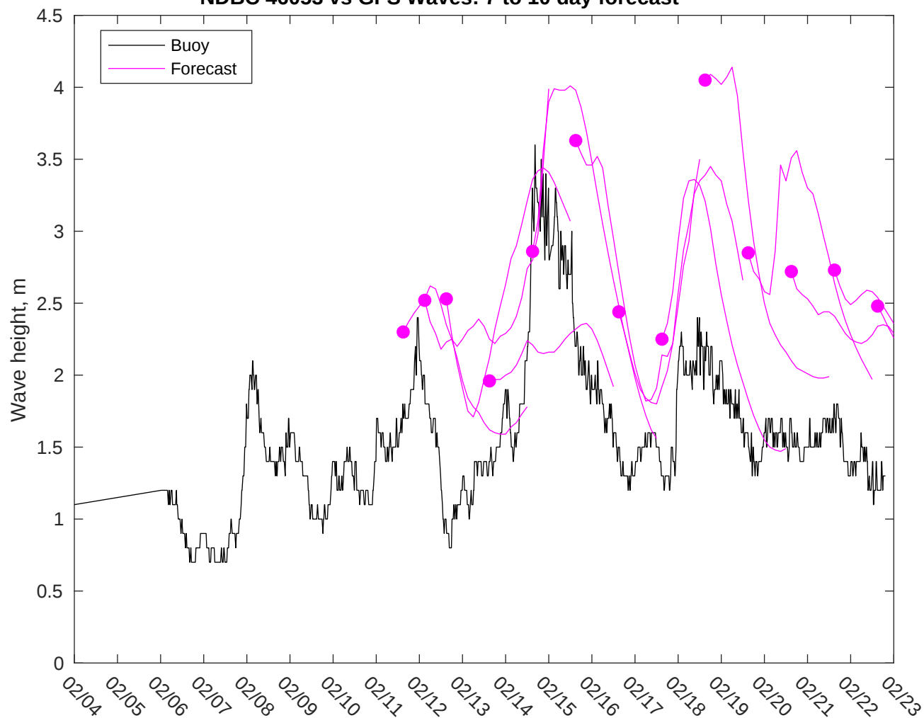
NDBC 46053 vs GFS Waves: 7 to 10 day forecast
