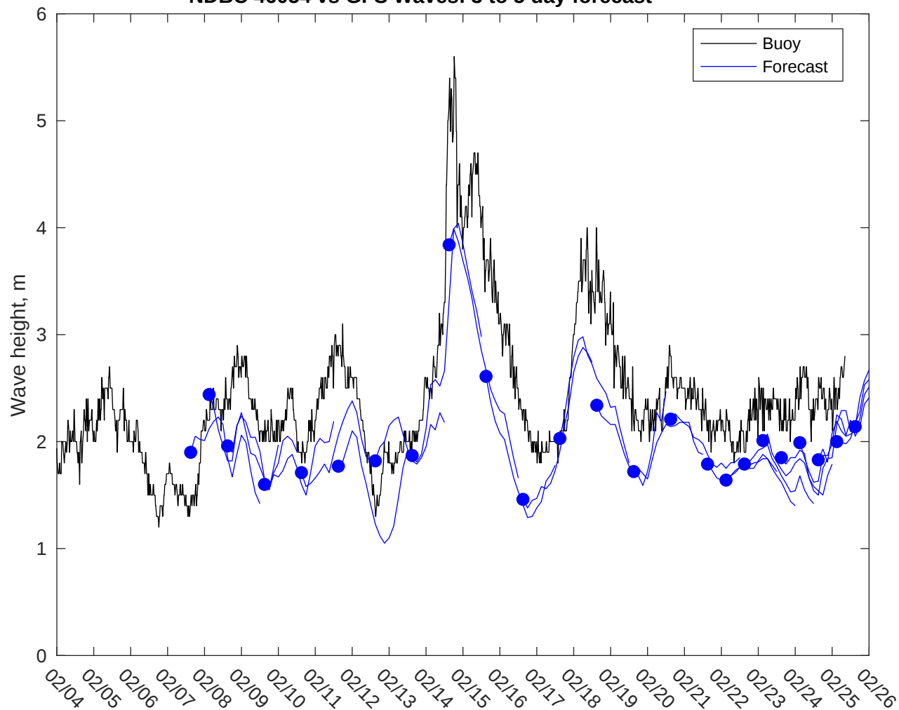
NDBC 46054 vs GFS Waves: 3 to 5 day forecast
