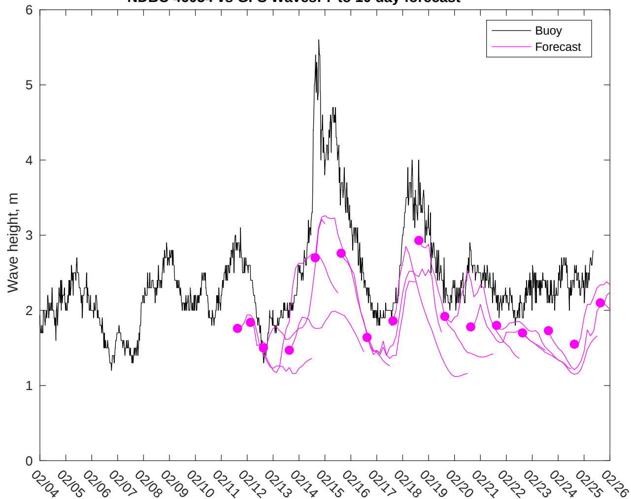
NDBC 46054 vs GFS Waves: 7 to 10 day forecast
